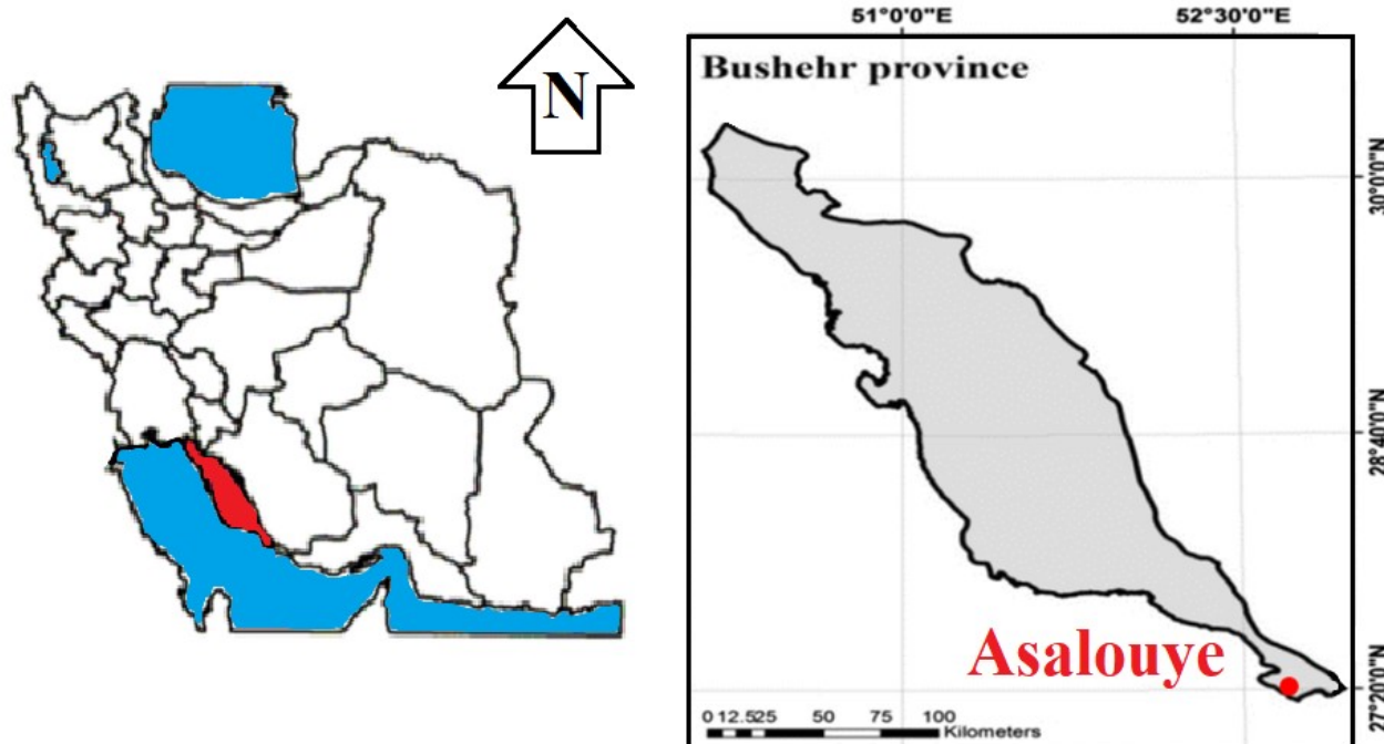
Fig. 1 Location of Asalouye region in Iran
